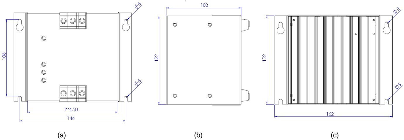
Şekil 7: Technical drawings for GAMMA-3010.
