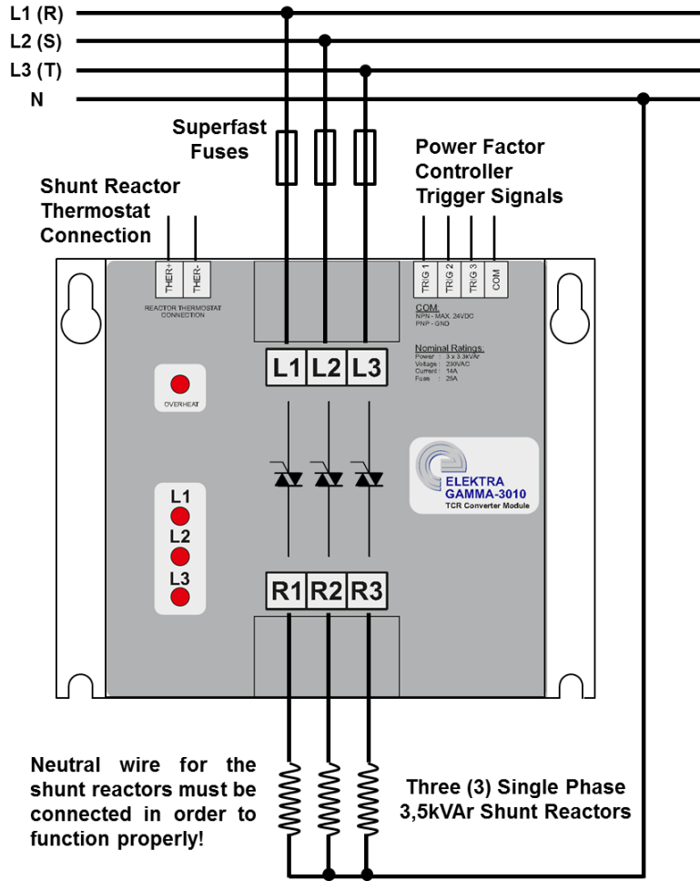
Figure 5: Wiring diagram of GAMMA-3010 modules. It is imperative to use a separate single phase shunt reactor for each phase, and the neutral connection of the shunt reactors must be connected to the neutral terminal on the GAMMA-3010 module and grid neutral wire.
