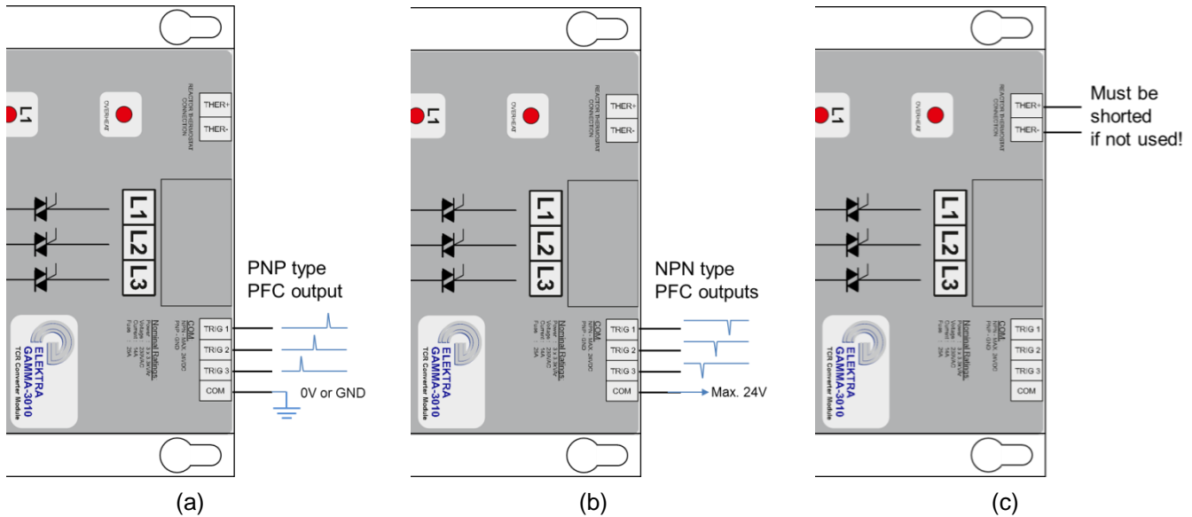
Figure 3: Connection and trigger signal illustration of GAMMA-3010 modules with (a) PNP and (b) NPN output type power factor controllers. If external thermostat connections will not be used, these terminals should be shorted as shown in (c).
