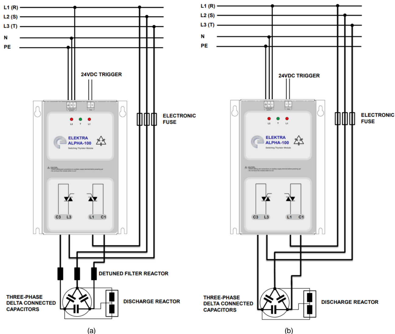
Figure 6: Recommended wiring diagram for ALPHA-100 module (a) with and (b) without a detuned filter reactor. Discharge resistors or reactors (shown) are imperative for frequent repetitive switching.
