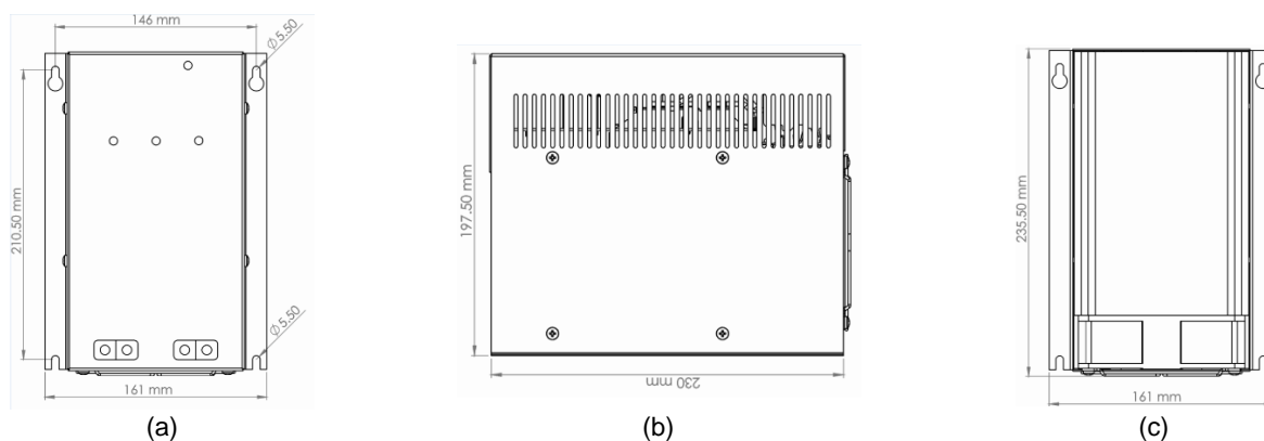
Figure 7: ALPHA-050 module technical drawings
