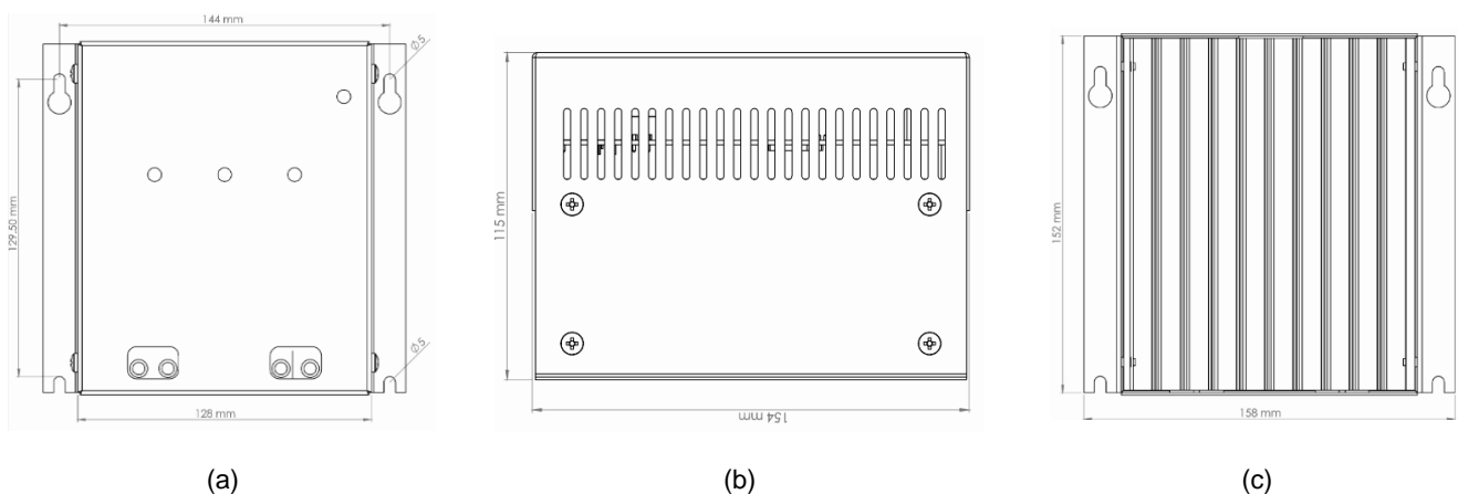
Figure 7: ALPHA-012-690V module technical drawings
