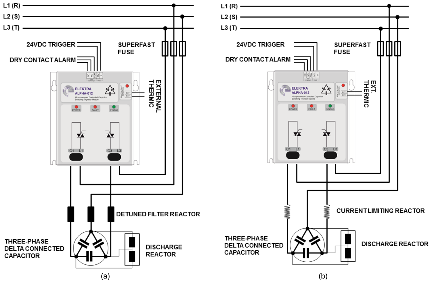
Figure 6: Recommended wiring diagram for ALPHA-012-690V module (a) with and (b) without a detuned filter reactor. Discharge resistors or reactors (shown) are imperative for frequent repetitive switching.
