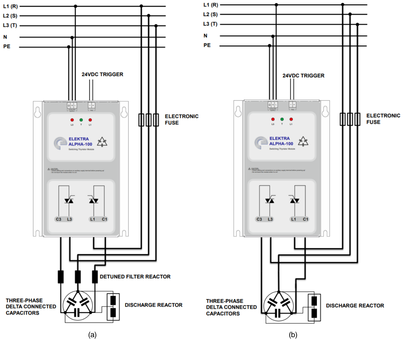
Figure 6: Recommended wiring diagram for ALPHA-100 module (a) with and (b) without a detuned filter reactor. Discharge resistors or reactors (shown) are imperative for frequent repetitive switching.
