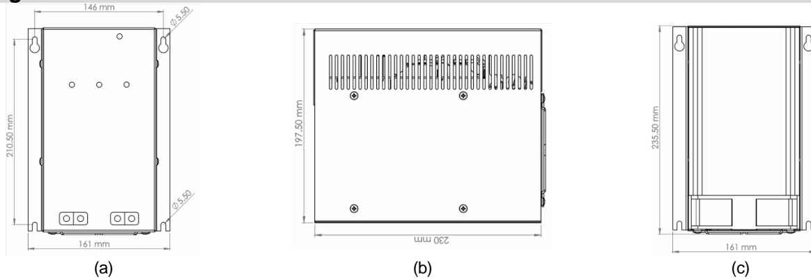
Figure 7: ALPHA-100 module technical drawings
