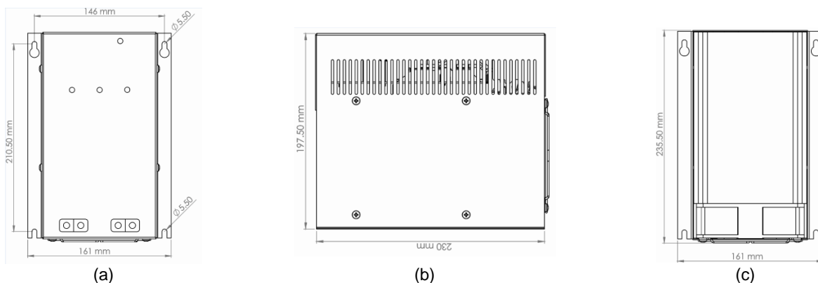
Figure 7: ALPHA-080 module technical drawings
