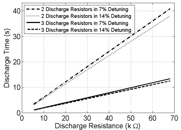
Figure 5: Discharge time vs. discharge resistance
