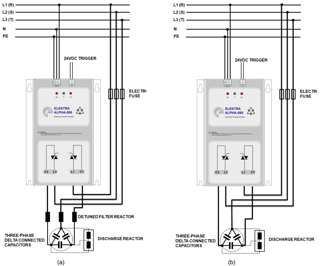
Figure 6: Recommended wiring diagram for ALPHA-080 module (a) with and (b) without a detuned filter reactor. Discharge resistors or reactors (shown) are imperative for frequent repetitive switching.
