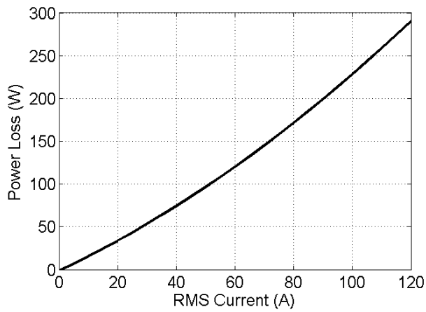
Figure 2: Power loss vs. RMS current
