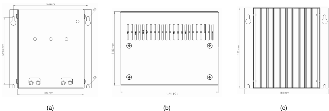
Figure 7: ALPHA-025 module technical drawings
