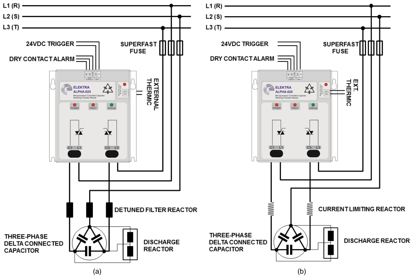
Figure 6: Recommended wiring diagram for ALPHA-025 module (a) with and (b) without a detuned filter reactor. Discharge resistors or reactors (shown) are imperative for frequent repetitive switching.
