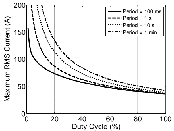
Figure 3: Absolute maximum current for repetitive switching operation (1 second period)
