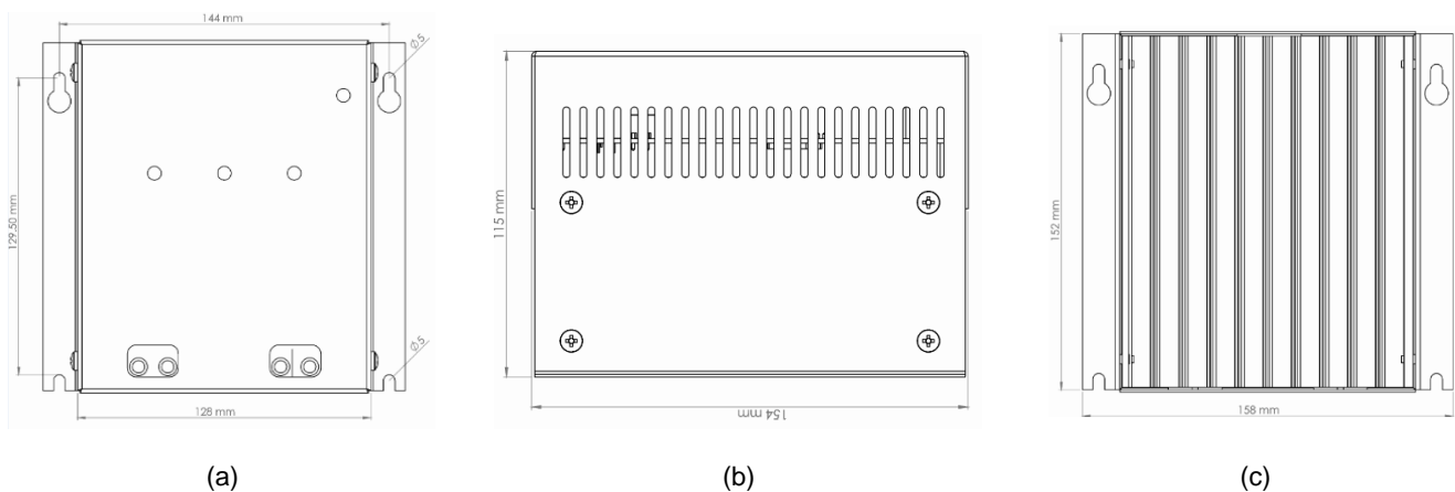
Figure 7: ALPHA-012 module technical drawings
