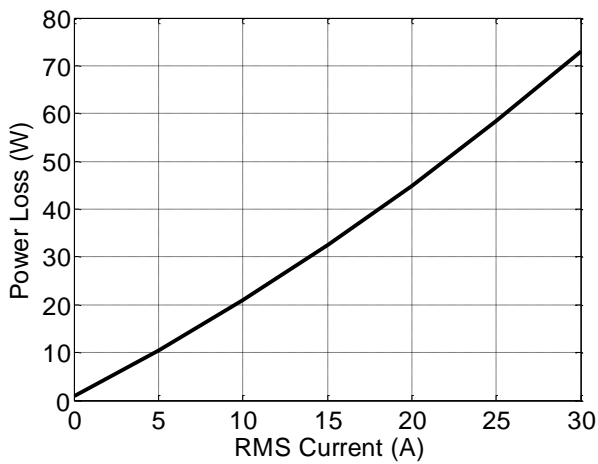
Figure 2: Power loss vs. RMS current
