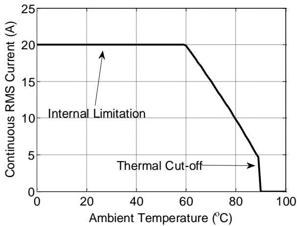
Figure 4: De-rating vs. ambient temperature under continuous operation (Safe operating area)
