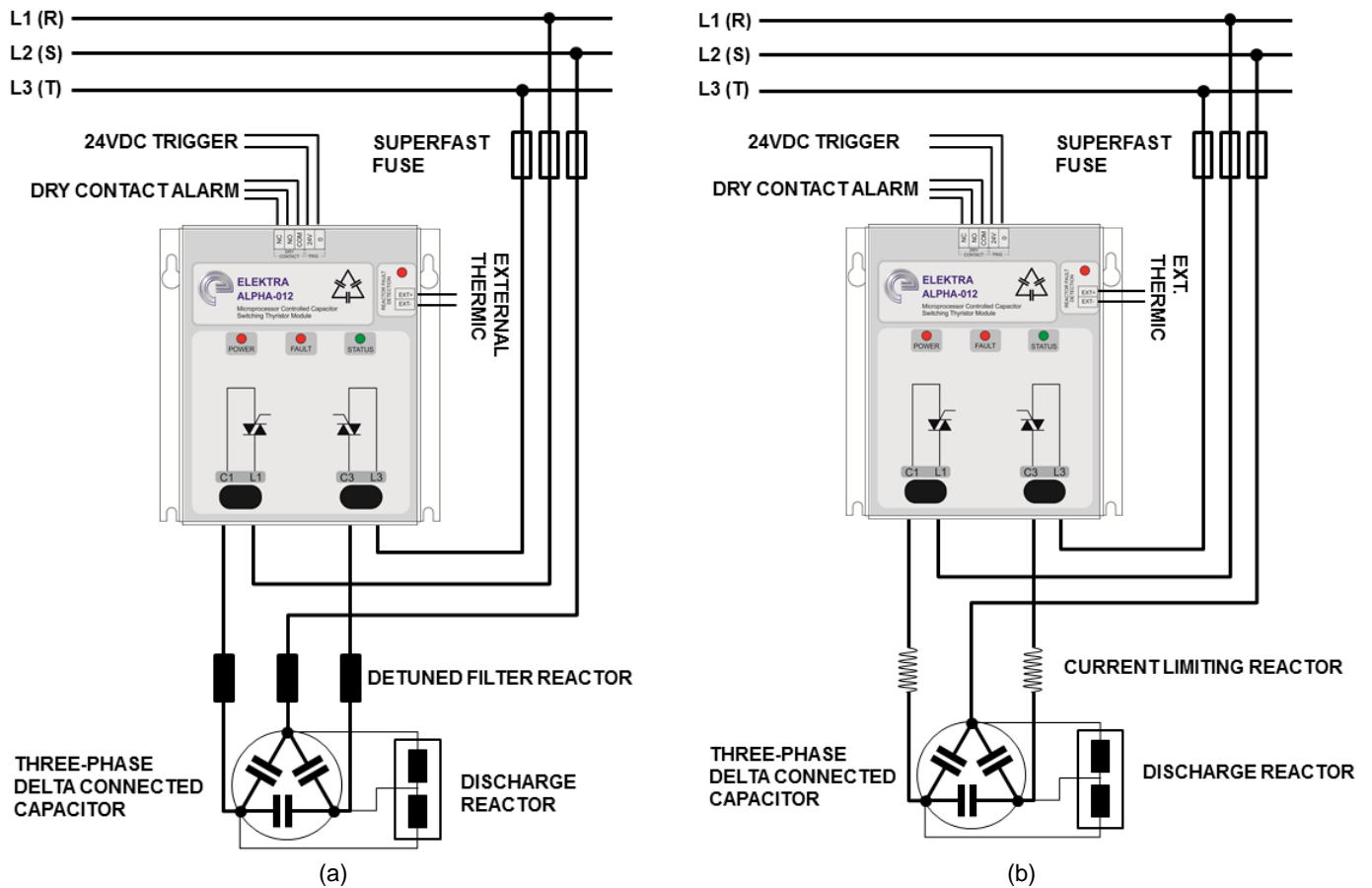
Figure 6: Recommended wiring diagram for ALPHA-012 module (a) with and (b) without a detuned filter reactor. Discharge resistors or reactors (shown) are imperative for frequent repetitive switching.
